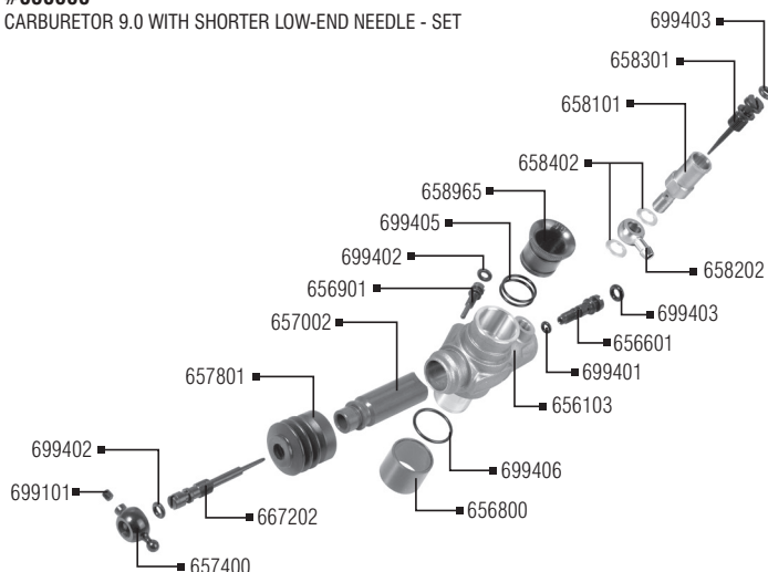
#656006 CARBURETOR 9.0 WITH SHORTER LOW-END NEEDLE - SET
